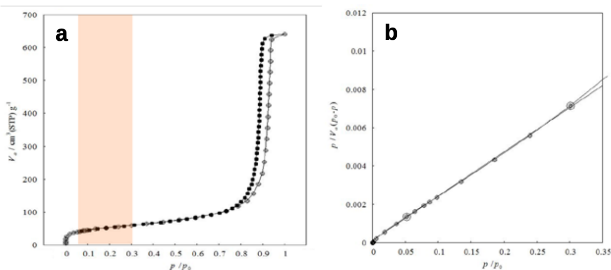
Fig. 3 – An example isotherm (a) and the respective BET plot (b) for a mesoporous material with a BET specific surface area of \sim 187 \text{ m}^2 \text{ g}^{-1} .
