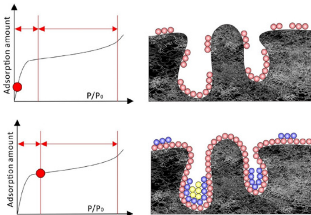
Fig. 2 – Isotherms and graphical representations depicting adsorption before (a) and at (b) the completion of the first monolayer. Note that second and third layers are produced in some regions before the completion of the monolayer.
